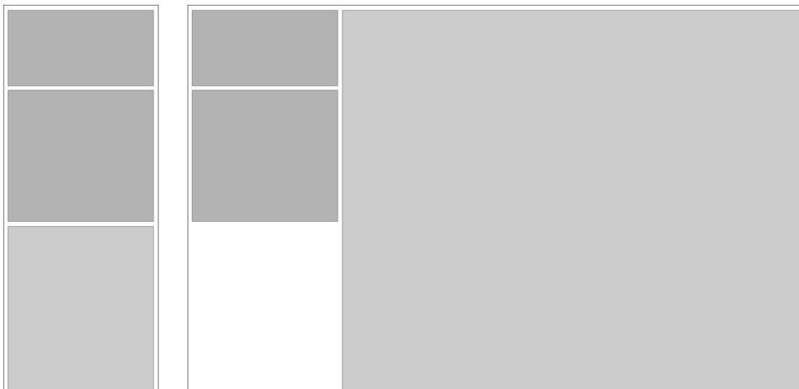
Figure 1. LINEARIZED LAYOUT.
