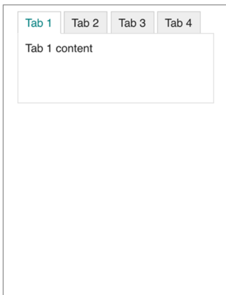
Figure 25. TABS.
