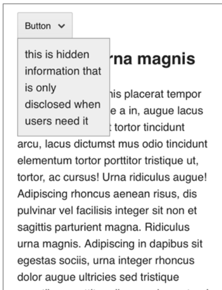
Figure 26. DROPDOWN.
