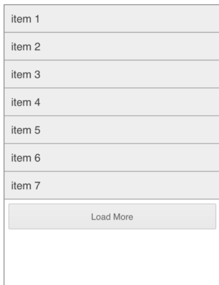
Figure 8. LINEARIZED MENU
