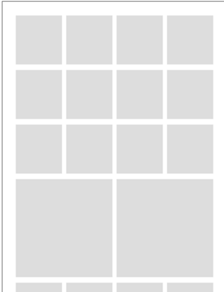
Figure 2. GRID LAYOUT.
